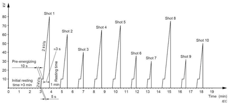
Figure A.1 – Example of a sequence of breakdown shots for determination of the breakdown voltage
