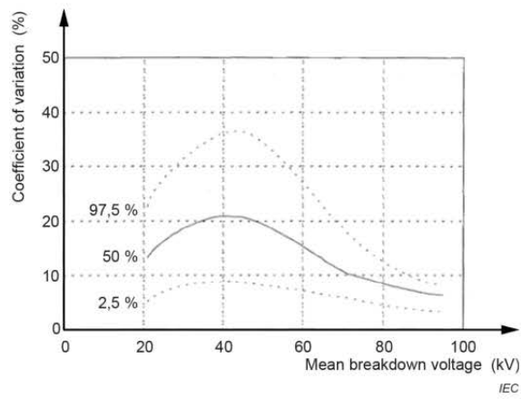
Figure 3 – Graphical representation of coefficient of variation versus mean breakdown voltage
